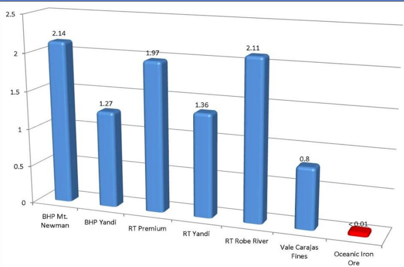
Alumina - % \text{AlO}_2\text{O}_3
