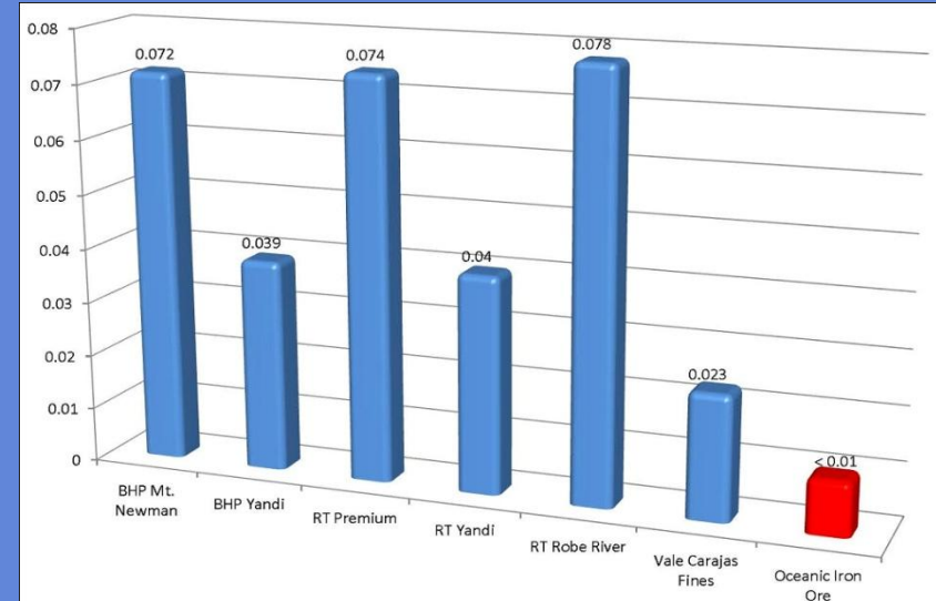
Phosphorus - %P
