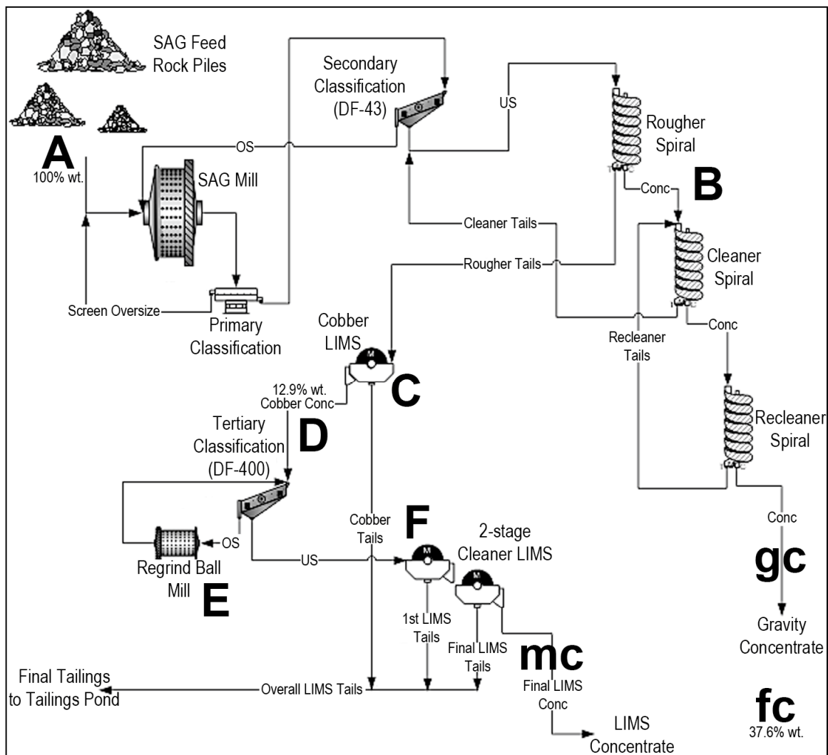
Figure 1 – Optimized Flowsheet
